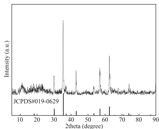
Fig. 2 X-ray diffraction patterns of \text{Zn}_{0.4}\text{Fe}_{2.6}\text{O}_4 NPs.
