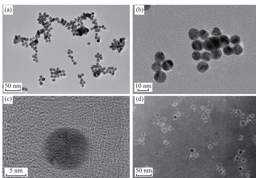
Fig. 3 Typical TEM images of (a)-(c) \text{Zn}_{0.4}\text{Fe}_{2.6}\text{O}_4 NPs (d) and \text{Zn}_{0.4}\text{Fe}_{2.6}\text{O}_4 -DSPE-PEG NPs.
