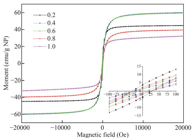
Fig. 1 Normalized magnetization curves of \text{Fe}_{3-x}\text{Zn}_x\text{O}_4 , the values of x were 0.2, 0.4, 0.6, 0.8, 1.0.
