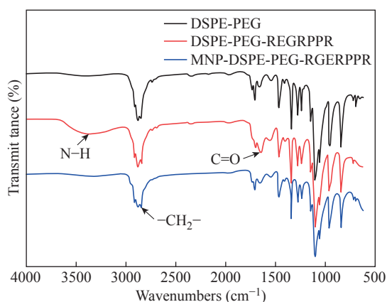
Fig. 4 FTIR spectrum of DSPE-PEG, DSPE-PEG-RGERPPR and \text{Zn}_{0.4}\text{Fe}_{2.6}\text{O}_4 -DSPE-PEG-RGERPPR NPs.
