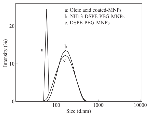
Fig. 5 Size distribution of \text{Zn}_{0.4}\text{Fe}_{2.6}\text{O}_4 , \text{Zn}_{0.4}\text{Fe}_{2.6}\text{O}_4 -PEG and \text{Zn}_{0.4}\text{Fe}_{2.6}\text{O}_4 -PEG-RGERPPR NPs.
